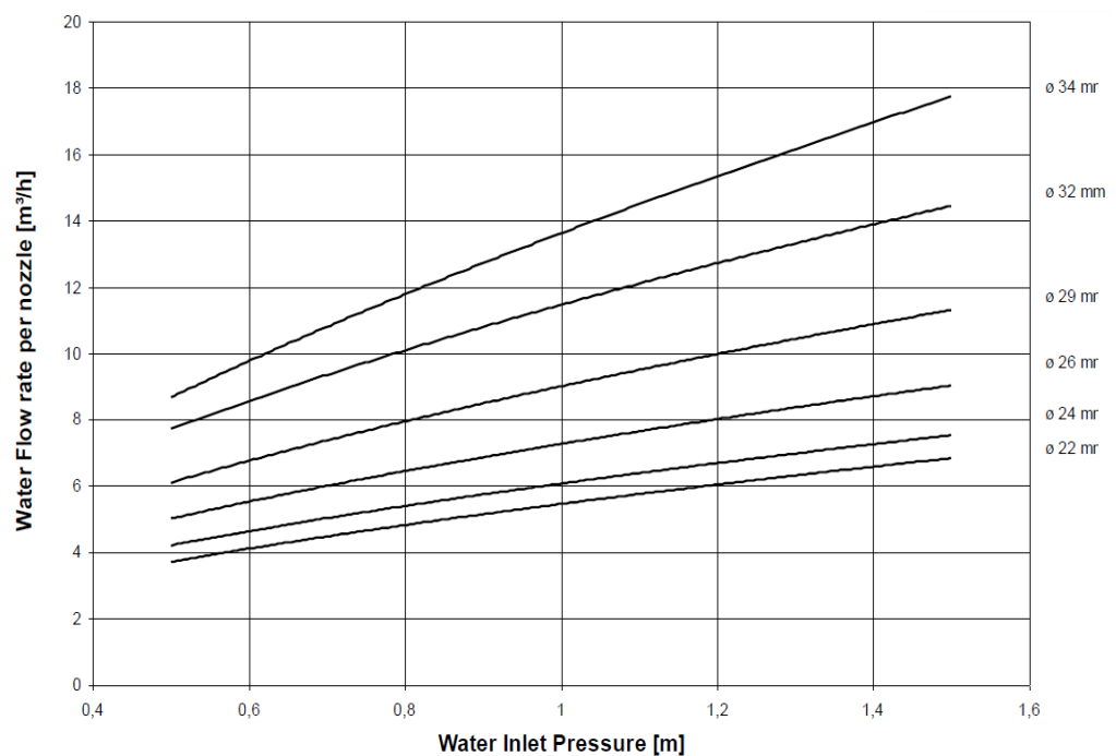
Sprayer characteristic
